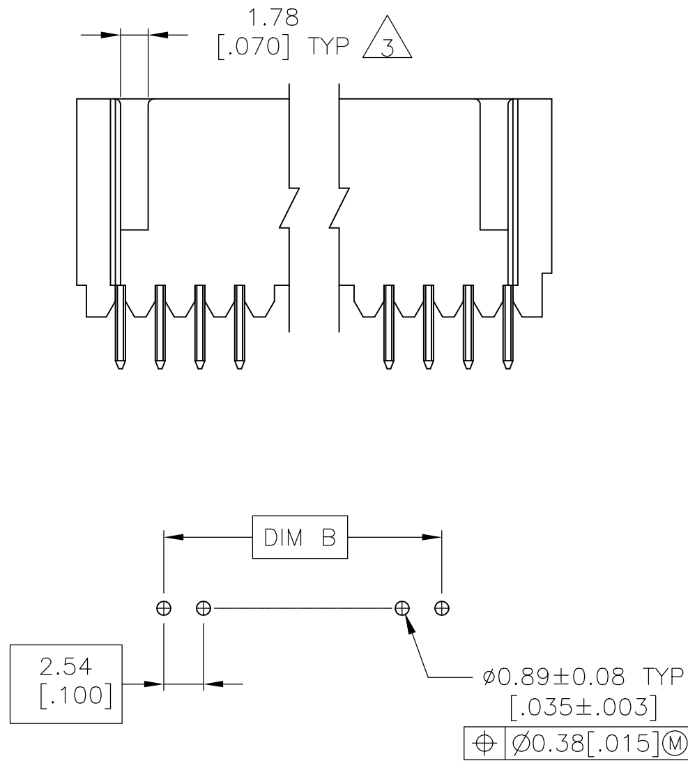
RECOMMENDED HOLE LAYOUT
