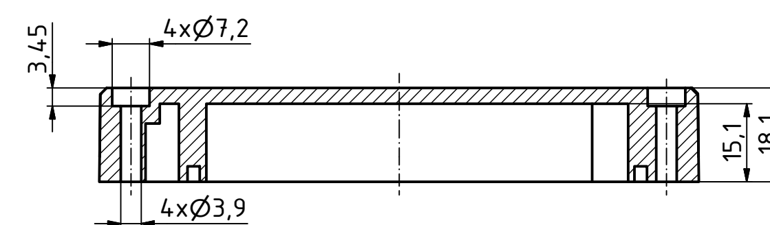
C-C (1:1)
