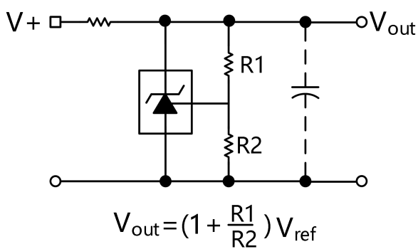
Figure 18. Shunt Regulator
