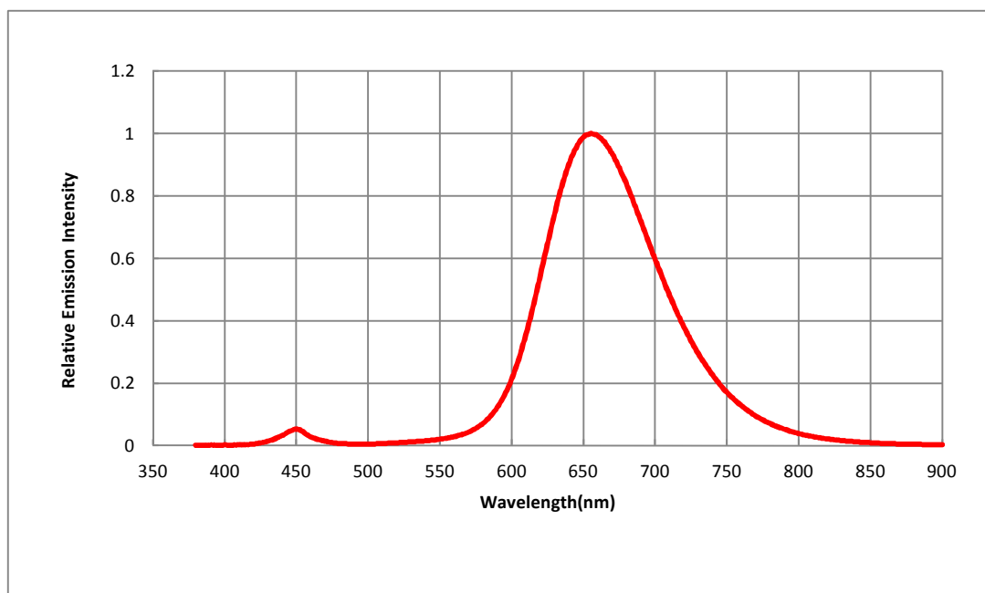
Fig 1-15 Spectrum Distribution光谱分布特性曲线
