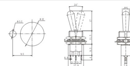
MTS-102-L1 ON-ON MTS-103-L1 ON-OFF-ON SPDT 3P
