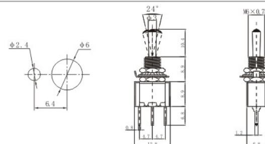
MTS-102-A2 ON-ON MTS-103-A2 ON-OFF-ON MTS-112-A2 ON-(ON) MTS-113-A2 ON-OFF-(ON) MTS-123-A2 (ON)-OFF-(ON) SPDT 3P
