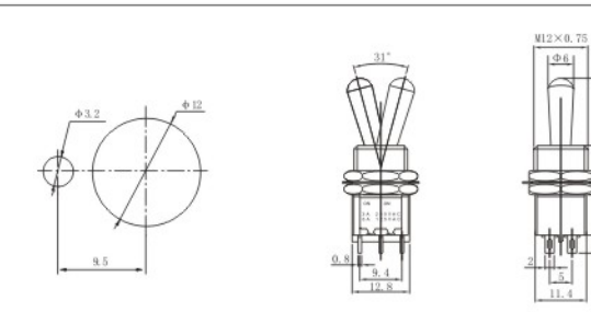
MTS-202-L1 ON-ON MTS-203-L1 ON-OFF-ON DPDT 6P
