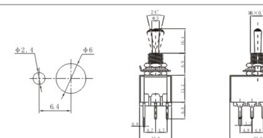
MTS-402-A2 ON-ON MTS-403-A2 ON-OFF-ON 4PDT 12P
