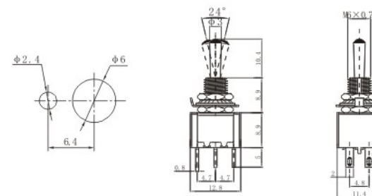
MTS-202 ON-ON MTS-203 ON-OFF-ON MTS-212 ON-(ON) MTS-213 ON-OFF-(ON) MTS-223 (ON)-OFF-(ON) DPDT 6P
