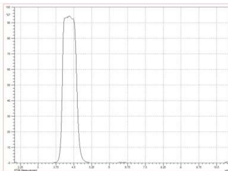
4.3um narrow band filter spectral curve
