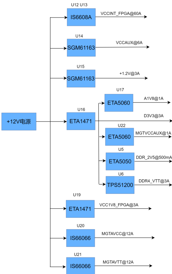
Figure 12: Power interface part in the schematic diagram
