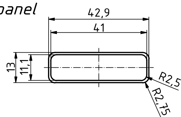
Frontplatte/ Front panel
