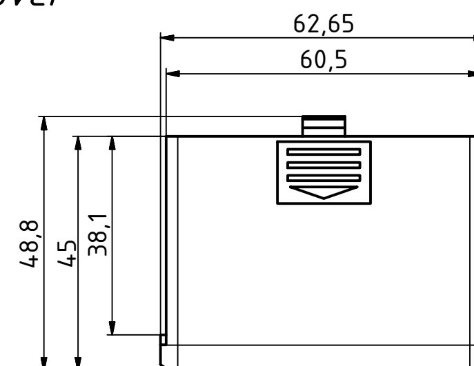
Batterie-Abdeckkappe/ Battery cover
