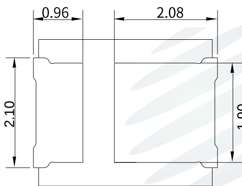
Fig.1-3 Bottom view
