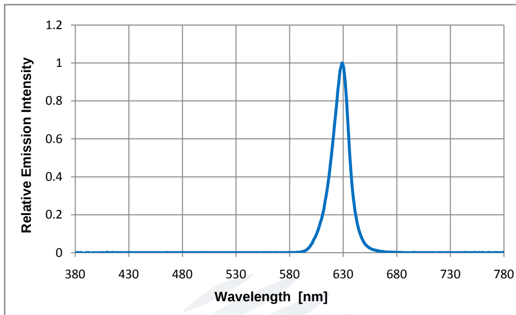
Fig 1-13 Spectrum Distribution
