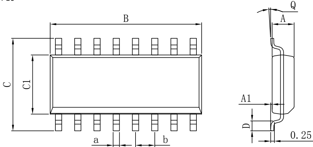
Dimensions In Millimeters
