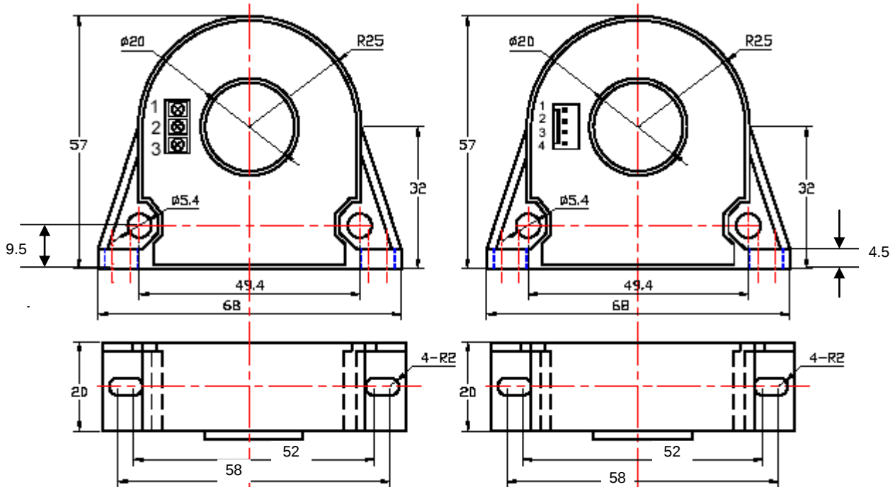
Screw Connector (P/N: CYHCS-D5Sxxxx) DG300-5.0 Screw terminal block
