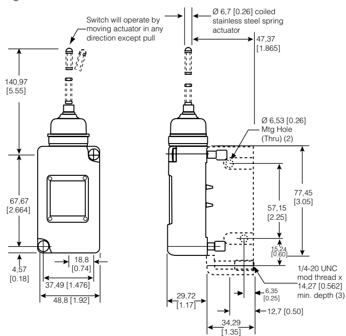
Figure 23. 208LS152 Dimensions
