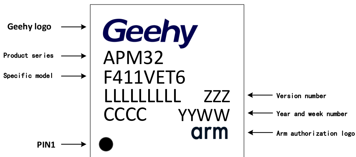
Figure 19 LQFP100 - 100 Pins, 14 x 14mm Diagram
