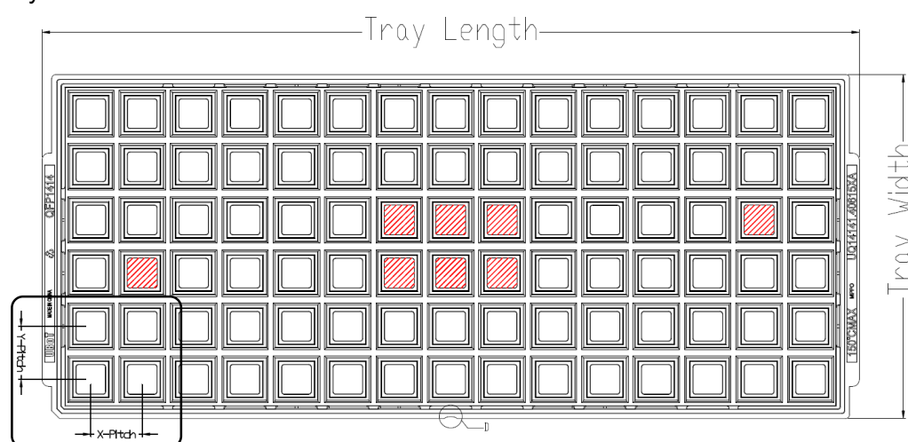
Tray Dimensions
