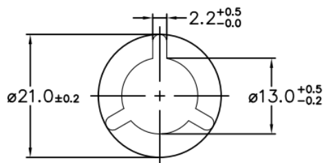
PRODUCT SPECIFICATION TAPE WIDTH φA ±2.0 φN ±2.0 W1 W2 (MAX) W3 E (MIN) 08MM 330 178 8.4 +1.5 -2.0 14.4 SHALL ACCOMMODATE TAPE WIDTH WITHOUT INTERFERENCE 5.5 12MM 330 178 12.4 +2.0 -2.0 18.4 5.5 16MM 330 178 16.4 +2.0 -2.0 22.4 5.5 24MM 330 178 24.4 +2.0 -2.0 30.4 5.5 32MM 330 178 32.4 +2.0 -2.0 38.4 5.5
