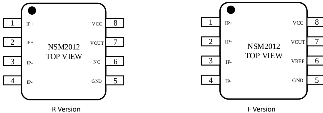
Figure 1.1 NSM2012 Package
