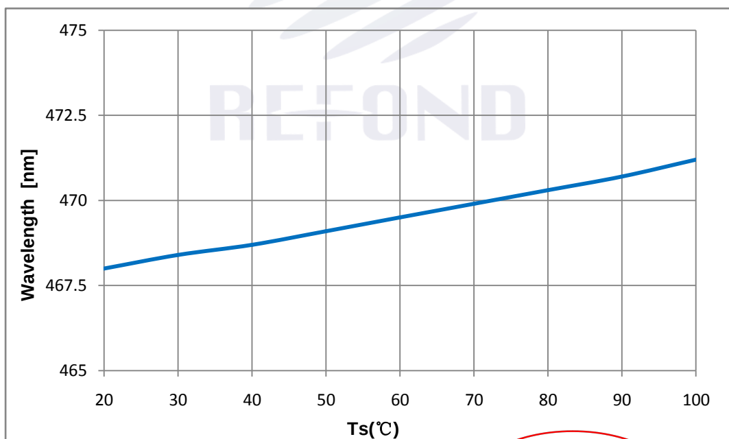
Fig 1-12 Wavelength Vs. Pin Temperature
