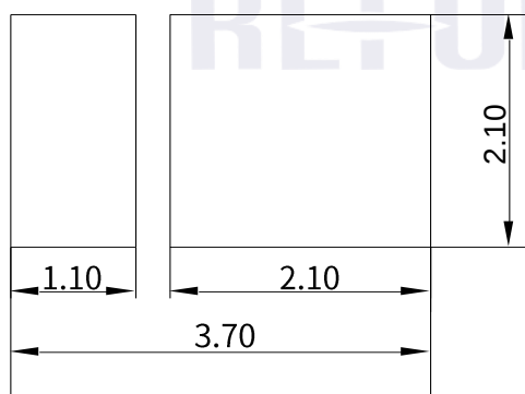
Fig.1-5 Soldering patterns
