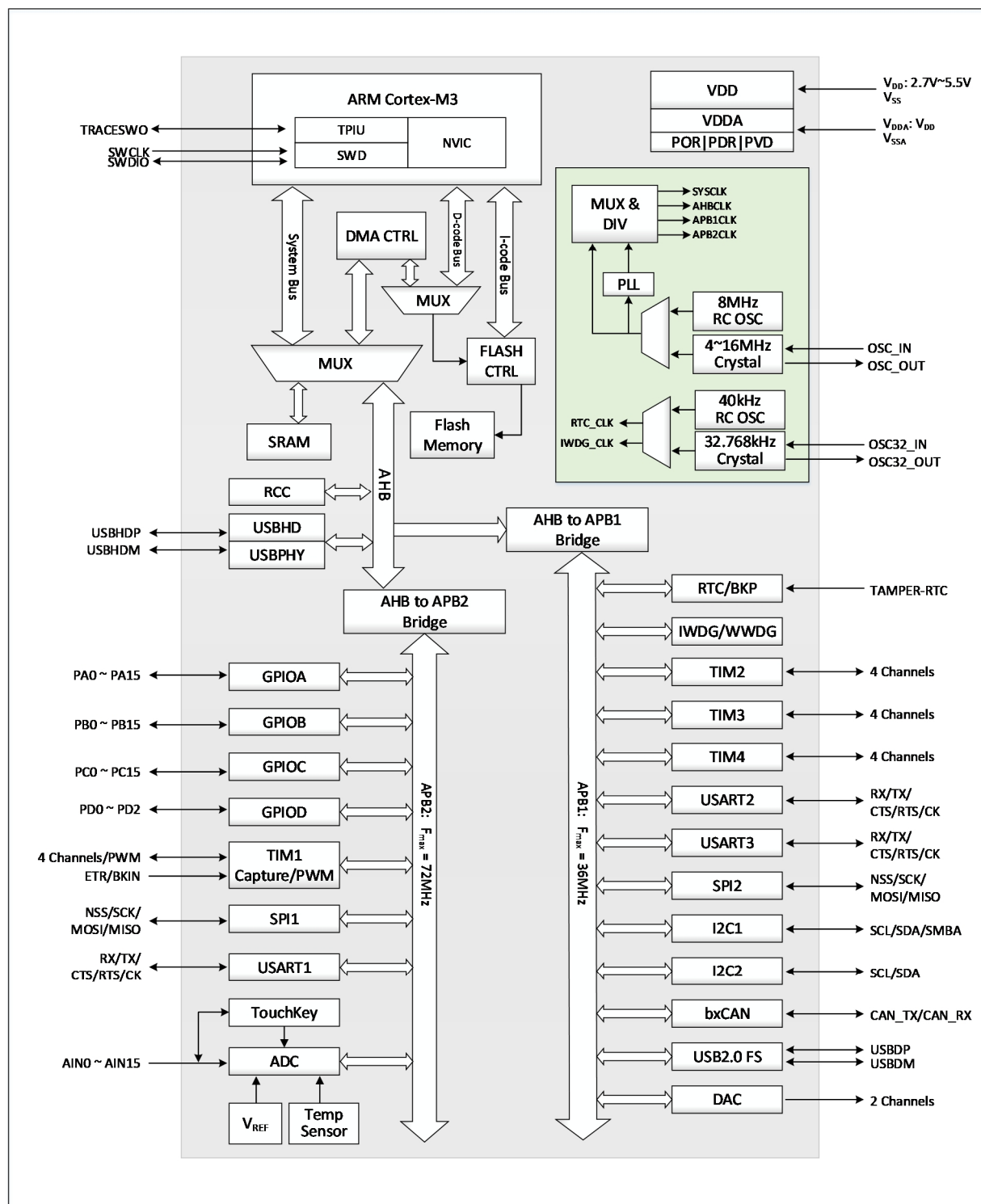
Figure 1-1 System architecture
