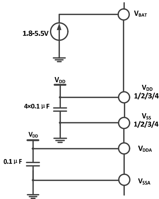
Figure 3-1 Power supply scheme
