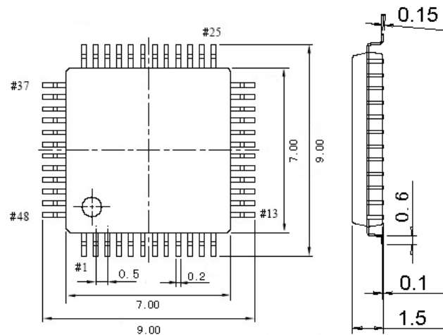
Figure 4-1 LQFP48 outline
