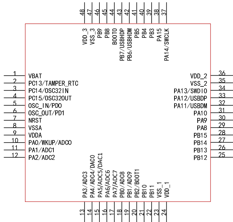
Figure 2-1 CH32F103Cx (LQFP48/QFN48X7) pinouts
