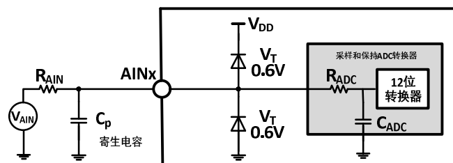
Figure 3-8 Typical connection diagram using the ADC
