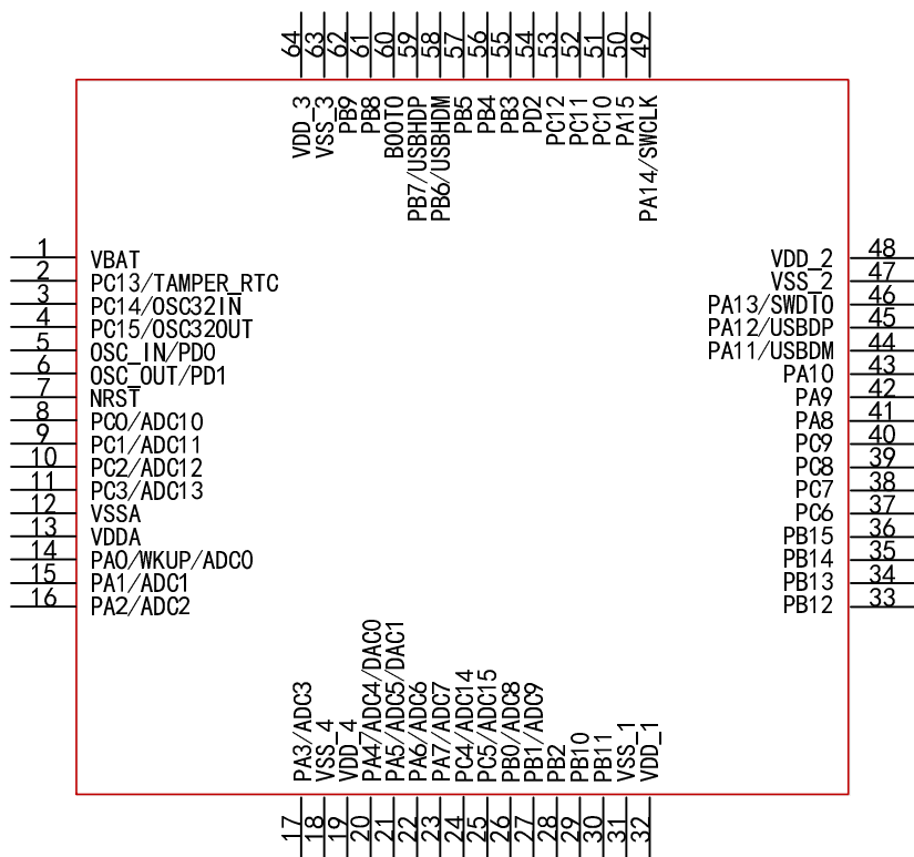
Figure 2-2 CH32F103Rx (LQFP64M) pinouts
