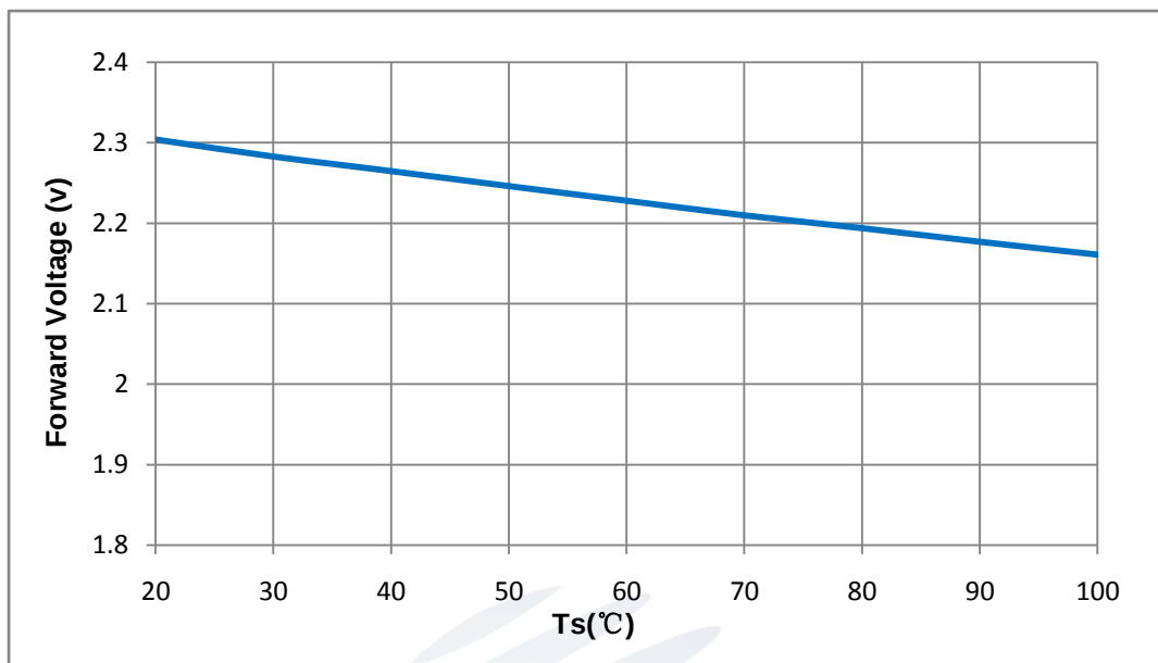
Fig 1-10 Forward Voltage Vs Solder Temperature 电压与管脚温度特性曲线
